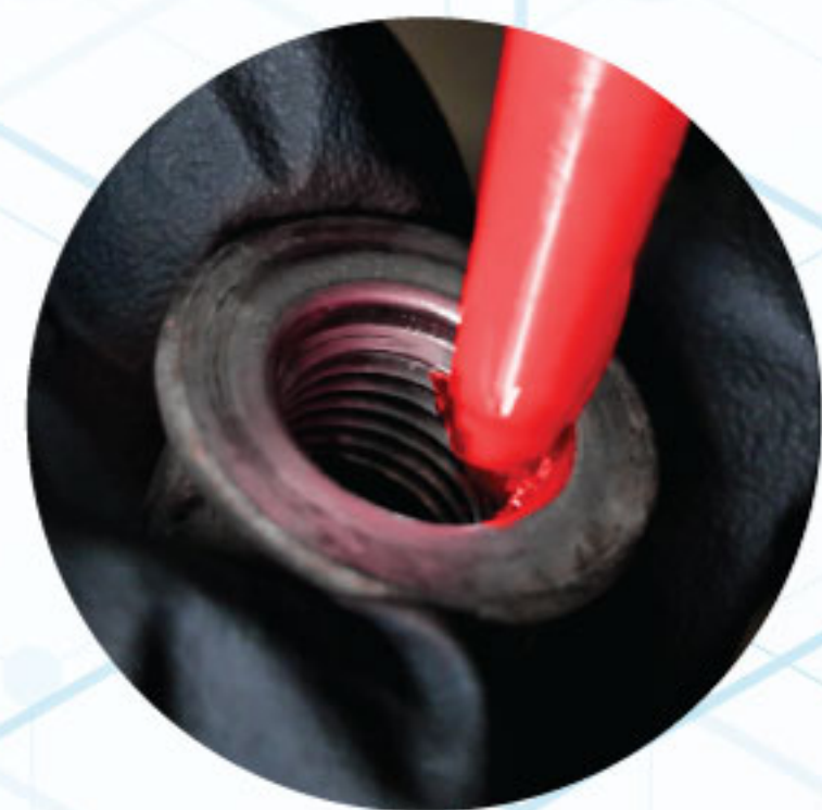
SEALING THREAD
